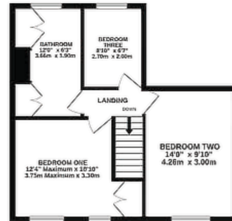
1ST FLOOR 452 sq.ft. (42.0 sq.m.) approx.
